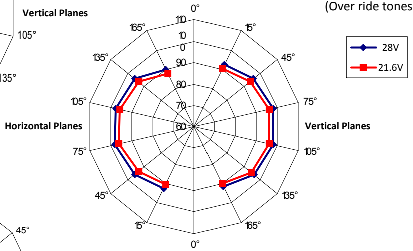
Continuous 800 Hz Tone (Over ride tones)
